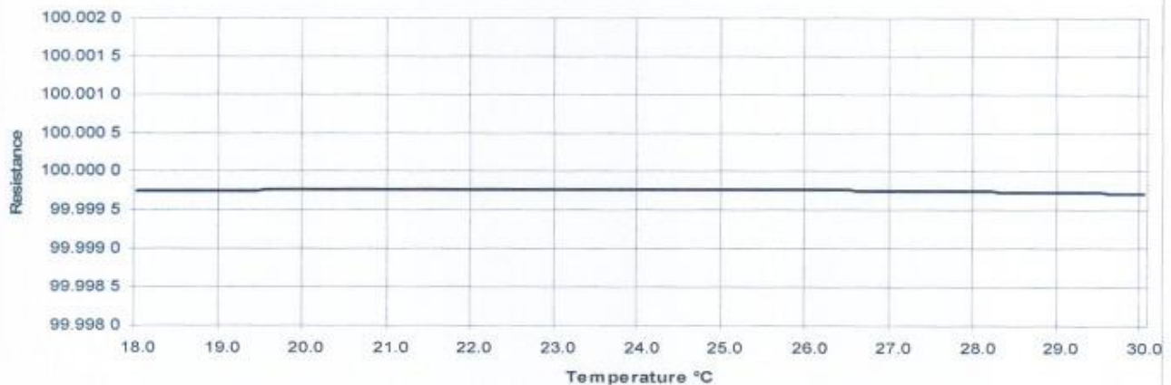
Resistance vs. Temperature Curve
